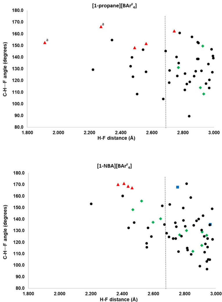
Fig. 4 Scatterplots of H \cdots F distance ( \text{\AA} ) vs. C-H \cdots F angle (degrees) for the [1-NBA] ^+ and [1-propane] ^+ cations within the octahedral arrays of neighbouring [BARF _4 ] ^- anions. The dashed vertical line indicates the sum of the van der Waals radii for H and F. a Data points correspond to two equivalent H \cdots F contacts.
