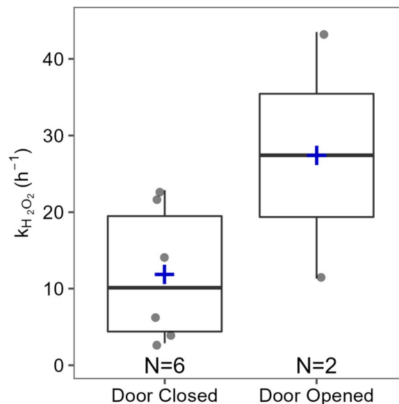
Fig. 4 Statistics of k_{H_2O_2} for regular cleaning of the near counter under different ventilation conditions. The box and whisker plots show the median (line), mean (blue marker), first and third quartiles (box), and minima and maxima (whiskers). The number under each box and whisker plot indicates the number of cleaning events for that condition.
