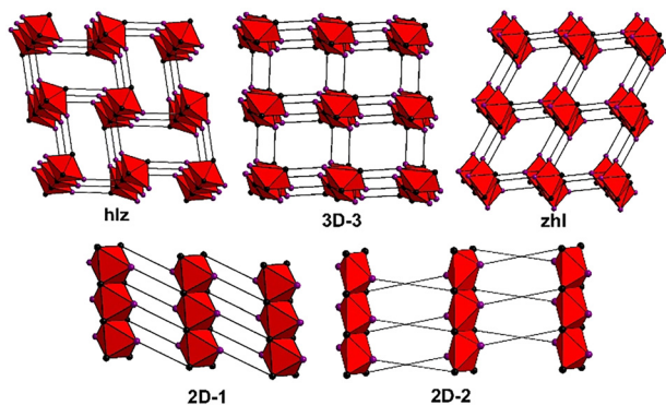
Scheme 2 Possible RBB topologies of ML_2 N-donor carboxylates.
