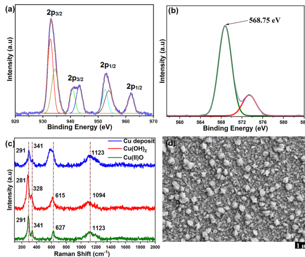
Fig. 4 XPS spectrum of the Cu deposit on FTO (after CPE) showing (a) Cu 2p and (b) Cu LMM regions. (c) Raman spectra of the Cu deposit, CuO and Cu(OH) 2 . (d) SEM image of the FTO electrode after 7 h of CPE.
