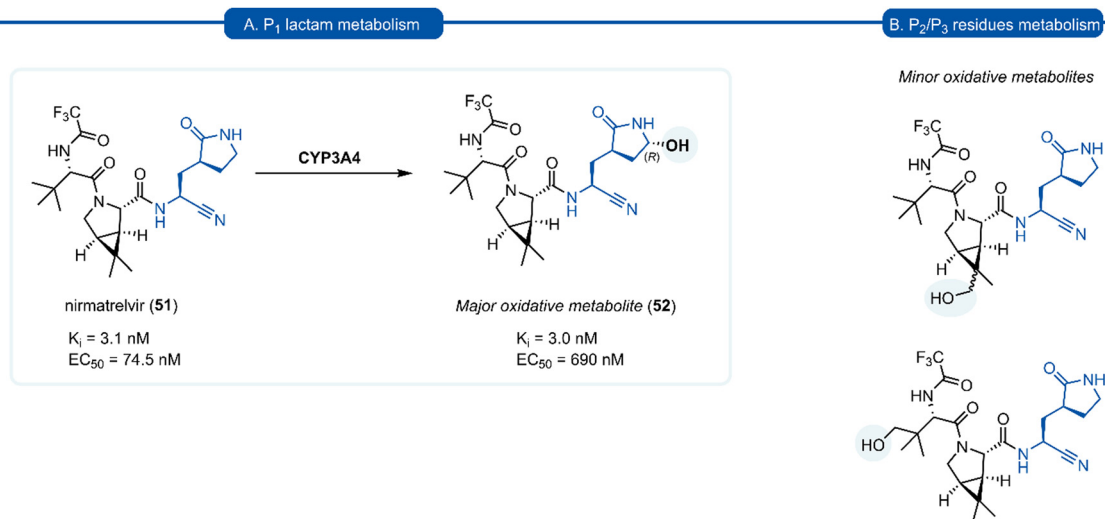
Scheme 3 (A) The primary route of metabolism of nirmatrelvir 51 via CYP3A4 hydroxylation of the P 1 (S)- \gamma -lactam moiety. (B) Minor metabolites products of nirmatrelvir 51 via CYP3A4 hydroxylation of the P 2 and P 3 moiety.
