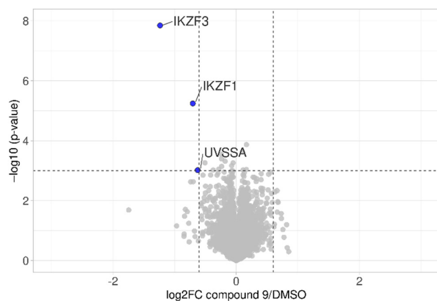
Fig. 4 diaPASEF quantitative proteomics for molecular glue 9 . MM.1S cells were treated with compound 9 at 0.1 \mu\text{M} for 3 h. Bioconductor's limma package was used to perform statistical analysis of degrader treatment compared to DMSO vehicle treatment. The identified proteins were plotted as \log_2 fold change (PROTAC/DMSO) versus -\log_{10} of the p -value. Proteins with -\log_{10} ( p -value) > 3 ( p -value < 0.001 ) and \log_2 fold change > 0.6 or < -0.6 (translating to 1.5-fold up- or down-regulation) were considered to have significantly changed in abundance. Data are the mean of biological duplicates.
