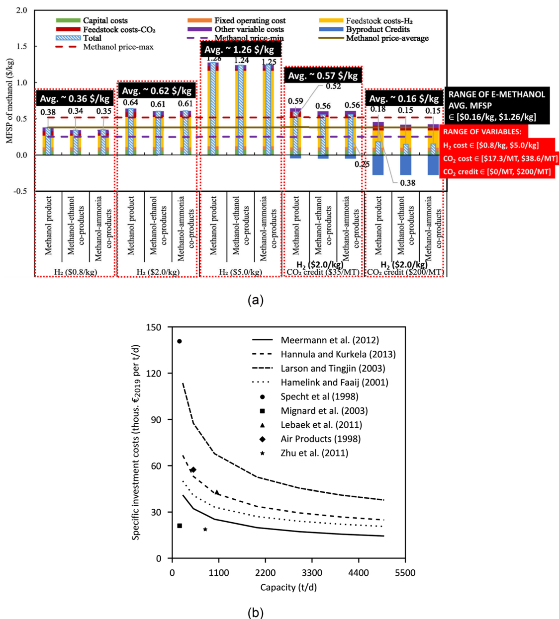
Fig. 13 (a) MFSP of e-methanol as a function of the \text{H}_2 production cost, \text{CO}_2 cost, and the credit for saved carbon, for a production capacity of 1190 MT per day. Adapted from ref. 78. (b) Cost of e-methanol production versus production plant capacity. From ref. 97.
