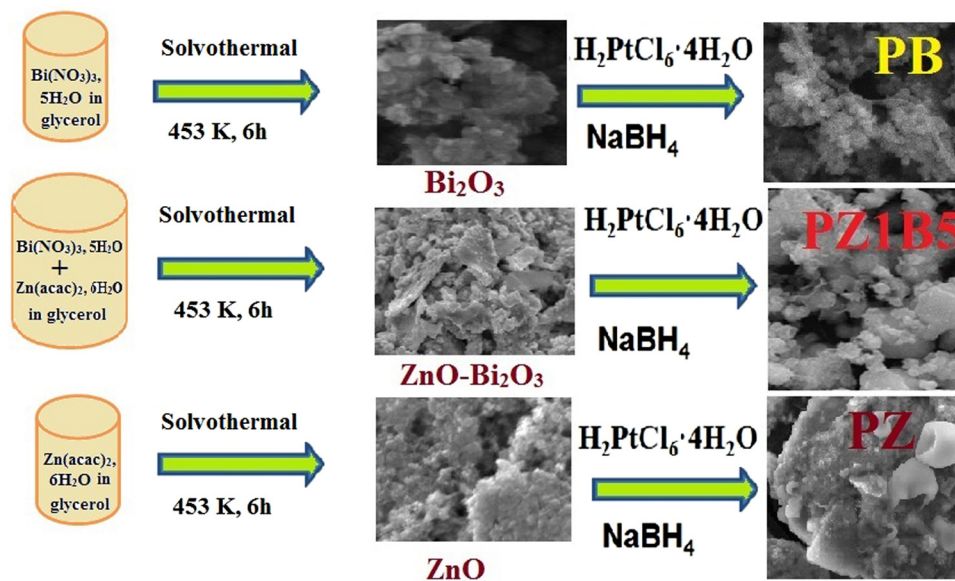
Scheme 1 The synthesis scheme of Pt–ZnO–Bi 2 O 3 heterojunction.
