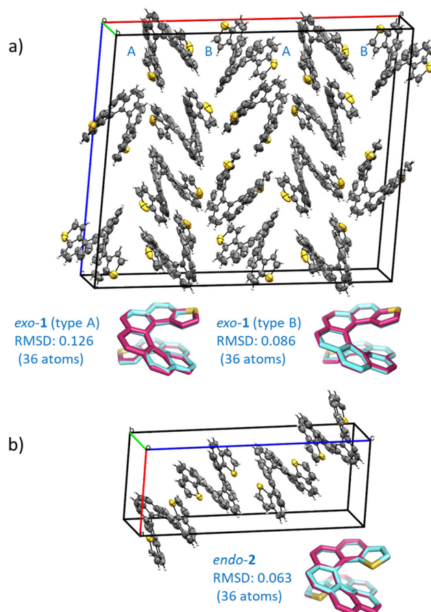
Fig. 1 (a) Crystal structure of the racemate exo -dithia[9]helicene ( 1 ): Monoclinic unit cell, space group C2/c , a = 33.075(4) , b = 9.8984(11) , c = 28.178(3) (Å); \alpha = 90^\circ , \beta = 94.890(2)^\circ , \gamma = 90^\circ ; Z = 16 ; CCDC number 2184340. The experimental structures of both molecular types found in the unit cell (A and B, reported in cyan) are overlapped with the calculated CAM-B3LYP/def2-SV(P) structures (in magenta) and shown below the unit cell; (b) crystal structure of the racemate endo -dithia[9]helicene- 2 : Monoclinic unit cell, space group P2_1/n , a = 9.712(2) , b = 9.709(3) , c = 25.072(6) (Å); \alpha = 90^\circ , \beta = 94.401(7)^\circ , \gamma = 90^\circ ; Z = 4 ; CCDC number 2184341. The experimental and calculated (CAM-B3LYP/def2-SV(P)) structures, reported in cyan and magenta respectively, are overlapped and shown below the unit cell. The root mean square deviation (RMSD, in Å) is calculated considering only the heavy atoms of an isolated dithia[9]helicene of ( M ) configuration for both isomers. For the crystal cells, ORTEP diagrams are shown with thermal ellipsoids drawn at 50% probability. The data was acquired at room temperature.
