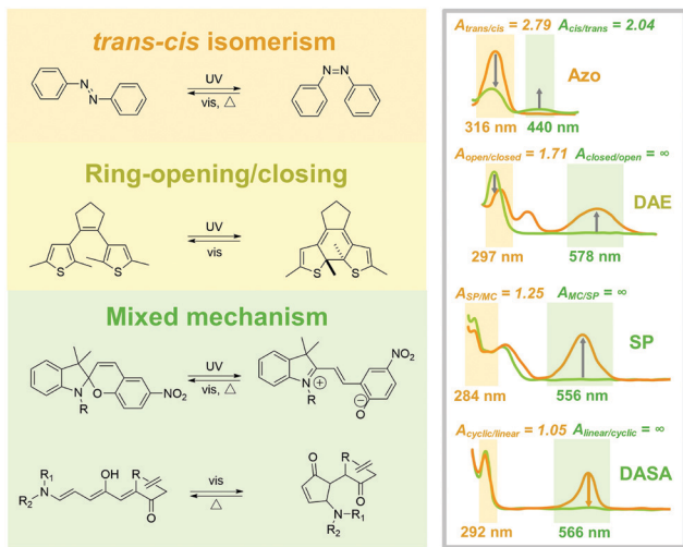
Fig. 2 Schematic illustration of chemical structure (left) and absorbance spectra (right) of the PSS of photoresponsive molecules (from top to bottom): azobenzene (Azo), dithienylethene (DAE), spiroopyran (SP) and donor-acceptor Stenhouse adduct (DASA).
