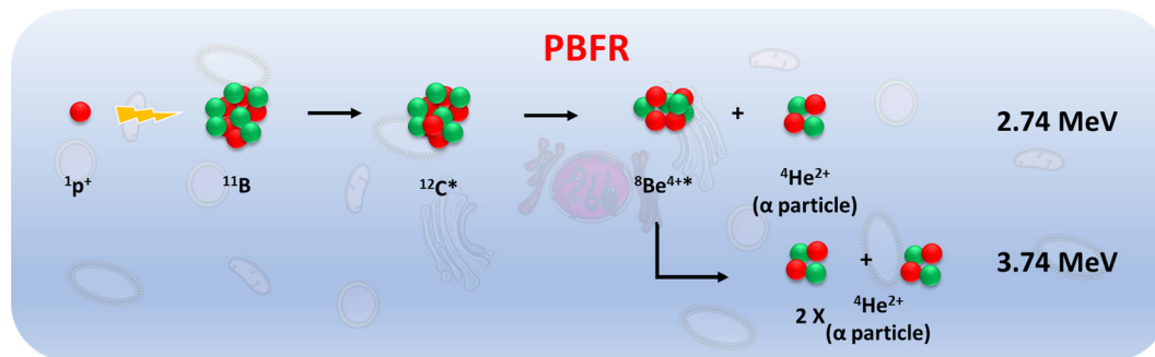
Scheme 2 Representation of the reaction between an energetic proton and {}^{11}\text{B} resulting in the generation of excited carbon {}^{12}\text{C} , which splits into a 2.74 MeV \alpha particle and a {}^8\text{Be} . Then, beryllium divides into two \alpha particles. Consequently, a total of three \alpha particles are generated by the proton boron reaction.
