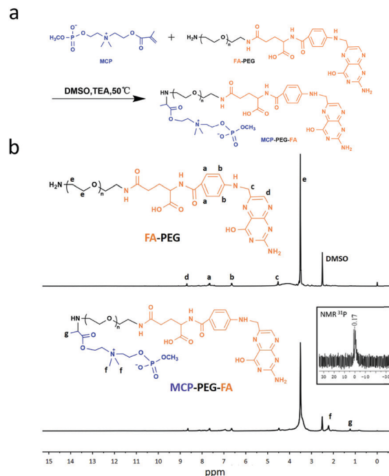
Fig. 2 (a) Synthetic route of MCP-PEG-FA. (b) ^1\text{H} NMR spectrum of FA-PEG, ^1\text{H} NMR spectrum and ^{31}\text{P} NMR spectrum of MCP-PEG-FA.
