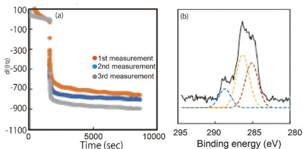
Fig. 2 Glycopolymer layer formation by adsorption of thiol-terminated pMan 200 . (a) Time course of frequency change of three different measurements in QCM by the adsorption of pMan 200 with 10 \text{ g L}^{-1} at 15 °C for 2 h. (b) XPS C (1s) spectrum of pMan 200 immobilized substrate after the adsorption of the glycopolymer and water rinsing.
