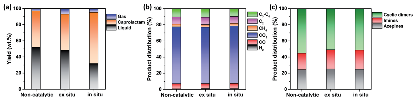
Fig. 6 (a) Yields of gaseous and liquid products, and caprolactam produced from the thermocatalytic conversion of FNW at 500 °C under an N_2 environment using SSWC- N_2 in different catalyst configurations; (b) distribution of gaseous products; (c) distribution of liquid products.
