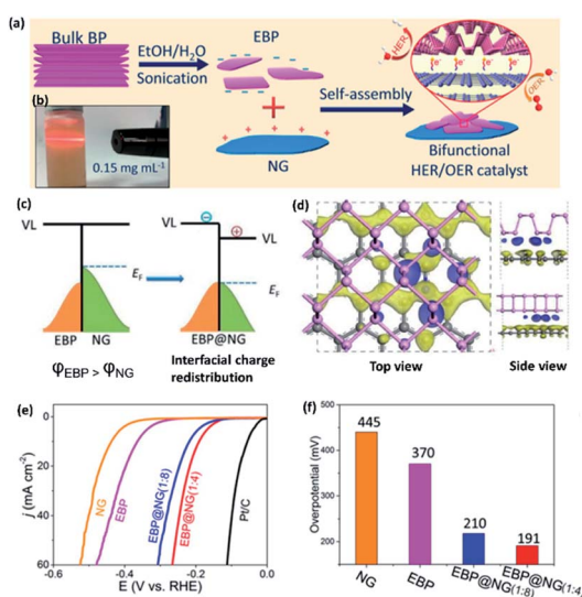
Fig. 7 (a) Schematic representation of liquid exfoliation of a BP crystal and preparation of EBP/NG composite (EBP = exfoliated BP; NG = N-doped graphene). (b) Optical image of EBP dispersion showing the Tyndall effect. (c) Illustration showing interfacial charge redistribution between EBP and NG at their Fermi levels. (d) Corresponding differential charge density map with the electron-rich and the hole-rich areas shown by blue and yellow regions, respectively. (e) LSV curves of various catalysts in 1.0 M KOH aqueous solution with the LSV curves of Pt/C and GCE are also given for comparison. (f) Corresponding bar diagram between the HER overpotentials at a current density of 10 \text{ mA cm}^{-2} and the mass ratio of EBP to NG in the EBP@NG composite. Reproduced with permission from ref. 6, © 2019 American Chemical Society.
