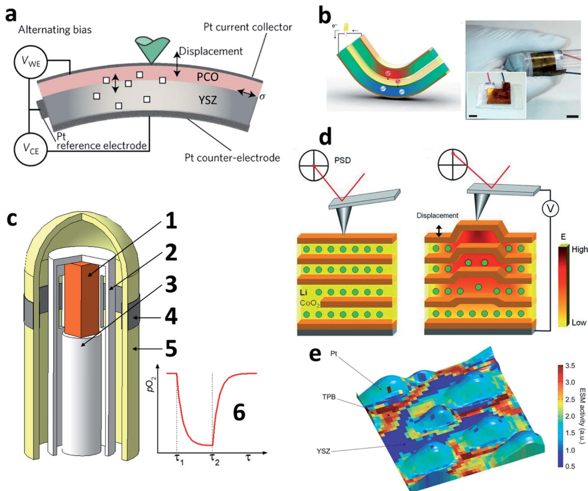
Fig. 10 (a) Illustration of the working principles of a thin film dynamic chemical expansion actuator: PCO – Ce_{0.9}Pr_{0.1}O_{2-\delta} , YSZ – yttria-stabilized zirconia. Adapted with permission from Springer Nature, J. G. Swallow, J. J. Kim, J. M. Maloney, D. Chen, J. F. Smith, S. R. Bishop, H. L. Tuller and K. J. Van Vliet, Dynamic chemical expansion of thin-film non-stoichiometric oxides at extreme temperatures, Nat. Mater. , 2017, 16 , 749–754, © 2017. 170 (b) A prototype of the mechanical energy harvester: (left) schematic view of the device design. The compressed region is illustrated in red while the tensile region is illustrated in blue. Lithium ions migrating from the compressed plate to the tensile plate are shown with arrows. The electrolyte soaked separator is drawn in yellow. (right) An image of the actual device with a bending unit. Both scale bars indicate 1 cm. Reprinted from S. Kim, S. J. Choi, K. Zhao, H. Yang, G. Gobbi, S. Zhang and J. Li, Nat. Commun. , 2016, 7 , 10146. 279 (c) Experimental apparatus for load-induced oxygen absorption measurements: 1 – oxide sample, 2 – sample holder, 3 – pushrod, 4 – YSZ electrolyte, 5 – Pt electrodes, 6 – typical pO_2 signal before ( \tau < \tau_1 ) and after ( \tau_1 < \tau < \tau_2 ) applying the load, and after releasing the load ( \tau > \tau_2 ). 280 (d) Electromechanical response of a battery material due to the correlation between Li-ion concentration and molar volume. (left) The scanning probe microscope tip is in contact with the sample surface (shown in layered LiCoO_2 as an example). (right) Locally applied electrical fields result in Li-ion redistribution in the probed volume, which leads to surface displacements. PSD – position sensitive detector. Reproduced from S. V. Kalinin and N. Balke, Adv. Mater. , 2010, 22 , E193–E209, with permission from John Wiley and Sons, © 2010. 28 (e) Overlay of electrochemical activity on the topography of the nanoparticles revealing the enhancement of activity along the triple-phase boundaries (TPB). ESM – electrochemical strain microscopy. This surface segment is around 270 \times 270 nm in size. Reprinted with permission from Springer Nature, A. Kumar, F. Ciucci, A. N. Morozovska, S. V. Kalinin and S. Jesse, Measuring oxygen reduction/evolution reactions on the nanoscale, Nat. Chem. , 2011, 3 , 707–713, © 2011. 291
