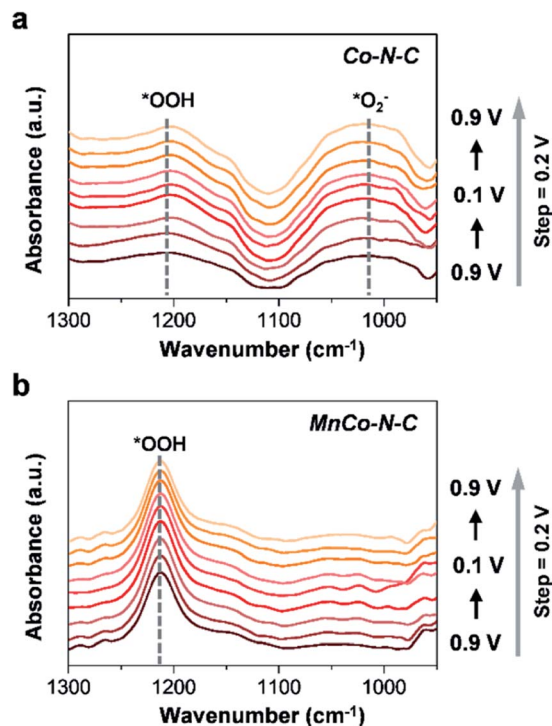
Fig. 5 (a and b) In situ ATR-SEIRAS spectra of Co-N-C and MnCo-N-C, respectively.
