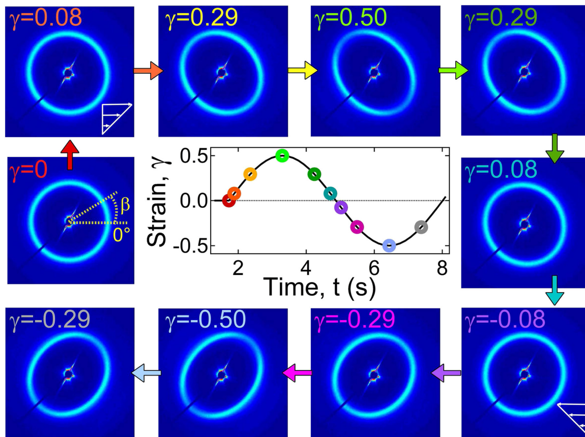
Fig. 10 Change of microstructure in a strain cycle for the A_{12}B_{96}A_{12}\text{-H} at room temperature. The strain ( \gamma ) cycle as a function of time at the center also indicates the \gamma -values at which 2D scattering patterns were obtained from RheoSAXS experiments (in a clockwise direction).
