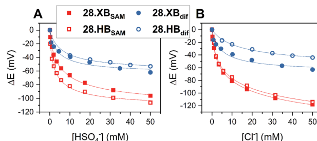
Fig. 29 Comparison of cathodic voltammetric shifts under diffusive conditions of 28.XB/HB dif (blue circles) and on the surface ( 28.XB/HB SAM (red squares)) in ACN/ \text{H}_2\text{O} 99 : 1 upon titration with (A) \text{HSO}_4^- and (B) \text{Cl}^- . Filled symbol represent the XB receptors while empty symbols represent the HB receptors. A pronounced surface enhancement was also observed for all other tested anions ( \text{Br}^- , \text{H}_2\text{PO}_4^- and \text{NO}_3^- ). Adapted from ref. 137 with permission from the Royal Society of Chemistry.
