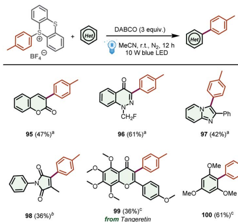
Scheme 4 Screening of other (hetero)aromatic cycles. (a) Reaction conditions: (hetero)aromatic cycle (0.1 mmol) was reacted with thianthrenium salt (0.2 mmol) in the presence of DABCO (3 equiv.) under 10 W blue LED irradiation. (b) 3-Methylene-1-phenylpyrrolidine-2,5-dione (0.1 mmol) is used as a substrate to react with thianthrenium salt (0.2 mmol) in the presence of DABCO (3 equiv.) under 10 W blue LED irradiation. (c) Thianthrenium salt (0.1 mmol) was reacted with (hetero)aromatic cycle (10 equiv.) in the presence of DABCO (3 equiv.) under 10 W blue LED irradiation.
