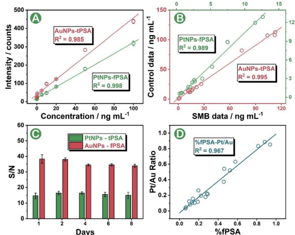
Fig. 4 (A) SMB nanoplatfom for simultaneous detection of fPSA and tPSA. (B) Data comparison between samples measured by using the SMB nanoplatfom and samples with known concentrations from the hospital. (C) Stability of the SMB nanoplatfom over 8 days. (D) Consistency between % fPSA and the Pt/Au ratio in 20 patients.
