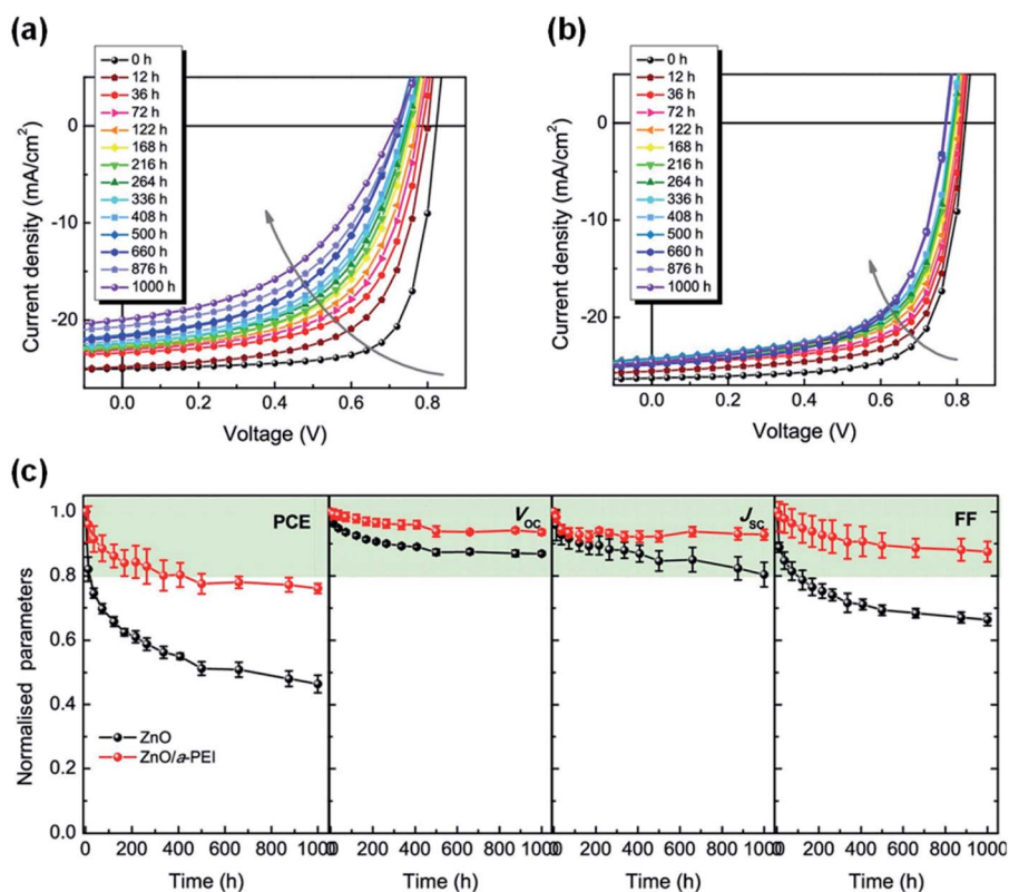
Fig. 19 Evolution of J-V characteristics under continuous AM1.5 G illumination in a nitrogen-filled glovebox with: (a) ZnO and (b) ZnO/a-PEI ETL; (c) evolution of photovoltaic parameters of the devices under continuous AM1.5 G illumination. Reproduced from ref. 49 with permission from the American Chemical Society, copyright [2021].
