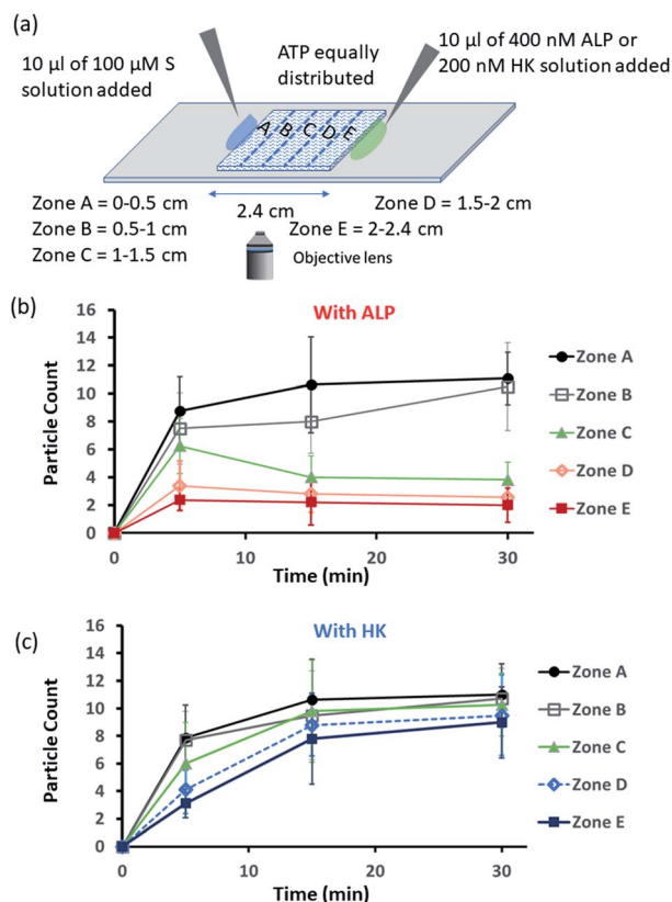
Fig. 5 (a) Schematic representation of the formation and evolution of fluorescent structures over time in a space having a concentration gradient of the surfactant (S), C 16 DPA·Zn 2+ , from the left side and of the enzyme (either ALP or HK) from the right side, and in which ATP and glucose and Mg(NO 3 ) 2 have been homogeneously distributed. Please see the ESI† for details of the experimental protocol. The experiments were performed by placing a square-shaped glass coverslip (2.4 cm × 2.4 cm) on a glass slide on which there was already a drop (20 μl) of ATP (20 μM) mixed with C153 (2.5 μM). The area under the coverslip was divided into five parts, and images were taken under a fluorescence microscope. (b and c) Absolute count of the aggregated fluorescent structures evolved in the different zones (A–E) after 5 and 30 min when ALP or HK was added from the right side. Images were taken under the fluorescence microscope at five different positions in each zone at 40× zoom, and the experiments were replicated three times to obtain an average of 30 images per zone.
