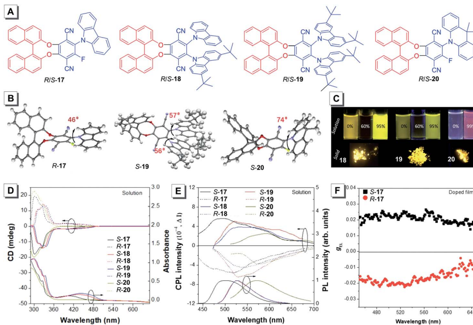
Fig. 20 (A) Molecular structures of 17–20. (B) Crystal structures of R -17, S -19, and S -20. (C) Fluorescence photos of S -18, S -19, and S -20 in THF and H 2 O mixtures with different water fractions and in solid powder under a UV lamp. (D) CD and (E) CPL spectra of R/S -17–20 in toluene. (F) Dissymmetry factors g_{EL} of R/S -17 in neat films. Adapted from ref. 68 with permission. Copyright 2018 Wiley-VCH.
