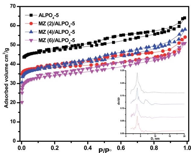
Fig. 2 \text{N}_2 adsorption-desorption isotherms of \text{MZn}(x)/\text{AlPO}_4\text{-5} nanocomposites, x = 0, 2, 4 , and 6. The inset is the pore size distribution of the prepared nanocomposites.
