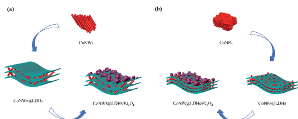
Fig. 11 Synthesis process of \text{CoNWs@CoAl-LDHs/Fe}_3\text{O}_4 (a) and \text{CoNPs@CoAl-LDHs/Fe}_3\text{O}_4 (b).
