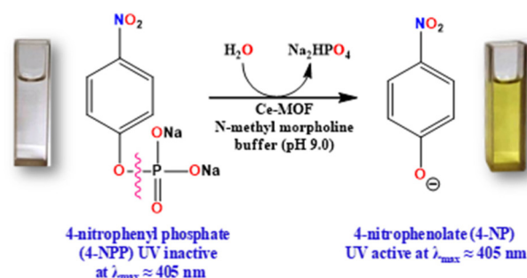
Scheme 3 Overview of Ce-MOF catalysts for the biomimetic hydrolysis of the phosphate ester (P–O) bond of (4-nitrophenyl)-phosphate hexahydrate (4-NPP).
