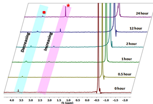
Fig. 10 ^{31}\text{P} -NMR spectra showing the species \text{Na}_2\text{HPO}_4 generated during the hydrolysis of 4-NPP in an \text{H}_2\text{O}:\text{D}_2\text{O} (90:10) medium at 25 °C. Assignments: ■ 4-NPP + N -methyl morpholine adduct, ★ \text{Na}_2\text{HPO}_4 (inorganic phosphate). Data were collected at 0 h, 0.5 h, 1 h, 2 h, 12 h and 24 h after the addition of the Ce-MOF.
