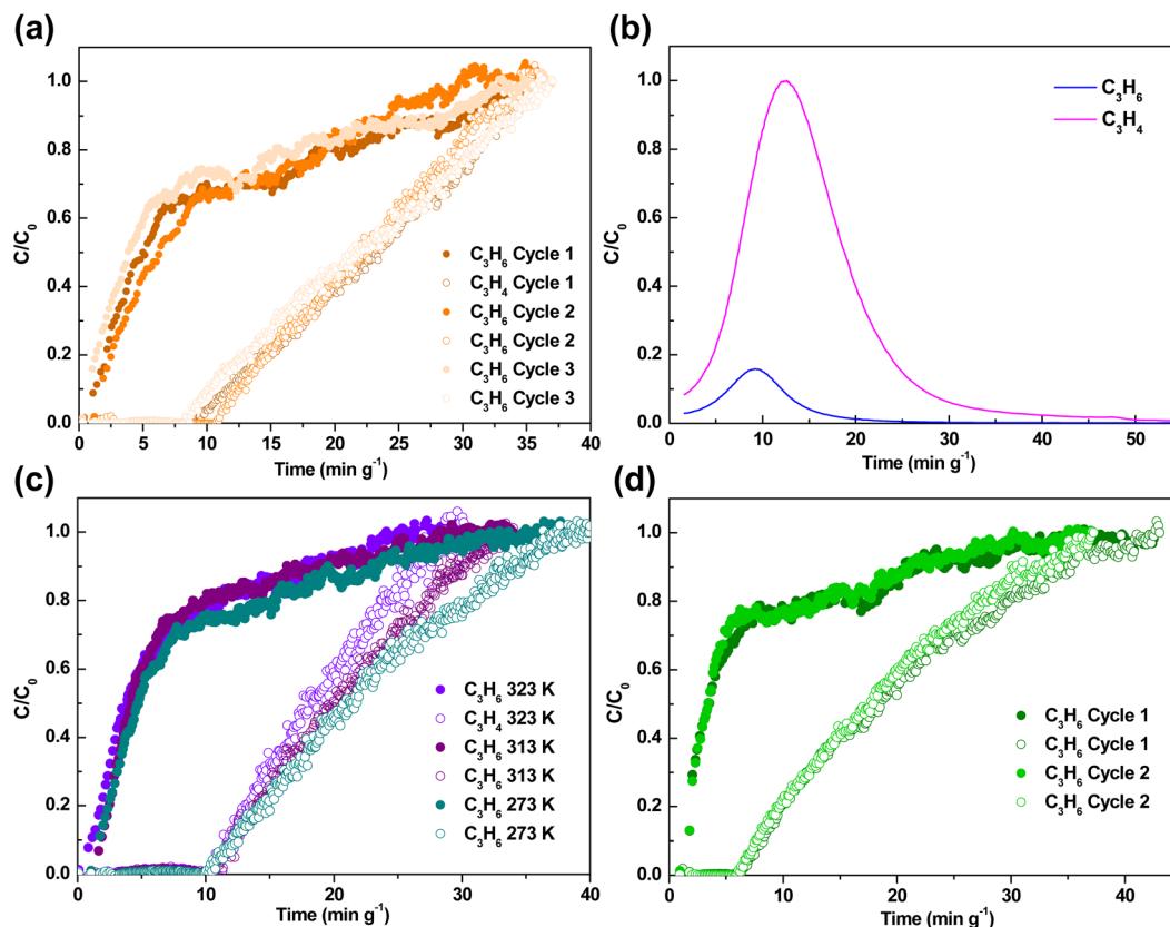
Fig. 5 Dynamic column breakthrough curves of BUT-306 for a binary C_3H_4/C_3H_6 (1:1, v/v) gas (a) at room temperature, (c) at 273, 313 and 323 K, and (d) under RH \approx 100% at room temperature, respectively. (b) The MS signal peaks of C_3H_4 and C_3H_6 at the outlet when the MOF column was purged with a He gas flow at 393 K after a breakthrough test at room temperature.
