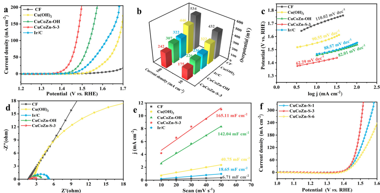
Fig. 6 OER performance test of electrocatalysts under alkaline conditions. (a) LSV polarization curves, (b) overpotential at 10 and 100 \text{ mA cm}^{-2} , (c) corresponding Tafel plots, and (d) Nyquist plots. (e) C_{dl} values and (f) LSV polarization curves at different times.
