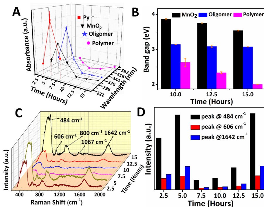
Fig. 2 (A) The absorbance and wavelength of UV-Vis absorption were plotted against the reaction time. (B) The band gap corresponding to the absorption peaks of the oligomer, the polymer, and \text{MnO}_2 plotted against the reaction time. (C) Raman spectra of PPY/ \text{MnO}_2 were recorded at varying time intervals of 2.5 to 15 hours. Bar plots showing (D) the intensity corresponding to the peaks of \alpha\text{-MnO}_2 and the backbone stretching mode of C=C bonds in PPY as a function of reaction time.
