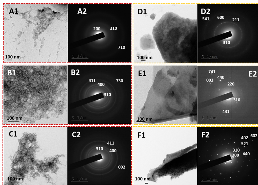
Fig. 3 High-resolution transmission electron microscopic images (series 1) and selected area electron diffraction images of PPY/ \text{MnO}_2 (series 2) recorded in a water/chloroform bisolvent medium at varying time intervals. The images A1 and A2, B1 and B2, C1 and C2, D1 and D2, E1 and E2, and F1 and F2 represent the reaction times of 2.5, 5, 7.5, 10, 12.5, and 15 hours, respectively.
