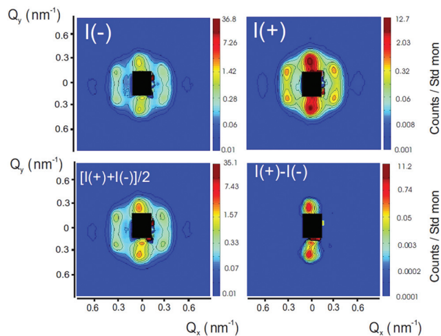
Fig. 19 SANS POL from frozen ferrofluids magnetite/oleic acid + oleylamine in decalin. In a homogeneous magnetic field of 0.2 T, a transition occurs to equal-spaced columns that exhibit hexagonal symmetry (reproduced from ref. 337 with permission from Am. Phys. Soc., copyright 2007).
