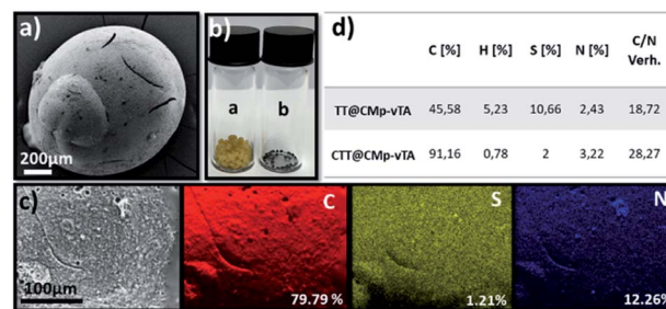
Fig. 3 Scanning electron microscopy image of TT@CMP-vTA (a), digital images of TT@CMP-vTA and CTT@CMP-vTA (a) and (b) (b), elemental mapping of CTT@CMP-vTA via EDX (c), and the combustive elemental analysis results of TT@CMP-vTA and CTT@CMP-vTA (d).
