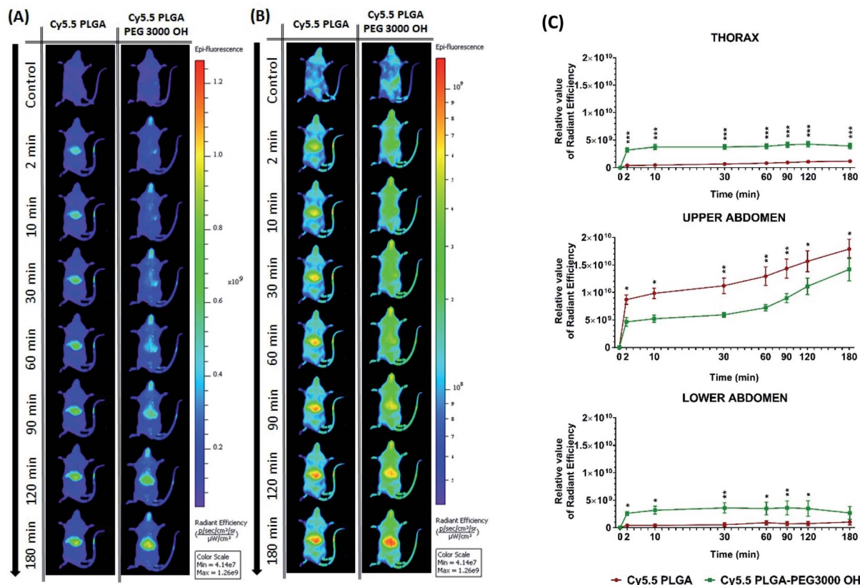
Fig. 5 In vivo real-time imaging and biodistribution of nanoparticles. (A and B) CD1 mice were injected via tail vein with 100 μL of PLGA NPs or PLGA-PEG NPs loaded with 20 mM Cy5.5/F12-TPB and were analyzed with Lumina XRMS imaging system at different time points ((A) radiant efficiency scale, (B) logarithmic scale). (C) The relative value of the fluorescence signal in three different area of the animal's body: thorax (lungs), upper abdomen (liver), lower abdomen (intestine and bladder) at different time points ( n = 4-5 ; * p < 0.05 ; ** p < 0.01 ; *** p < 0.001 ). For area determination in the mice body see Fig. S4.†
