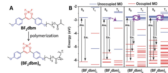
Fig. 2 Polymerization-enhanced lifetime of excitons. (A) Chemical structures of BF_2dbm and (BF_2dbm)_n . (B) Calculated selected molecular orbital energy diagrams for the S_0 and T_1 states of (BF_2dbm)_n . (B was reprinted with permission from ref. 30, Copyright 2015, Wiley-VCH Verlag GmbH & Co.)
