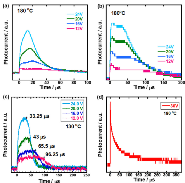
Fig. 2 Transient photocurrent curves for holes in the N* phase of (a) compound 1 at 180 °C, (b) 2 at 180 °C, (c) 3 at 130 °C, and (d) 4 at 180 °C. The sample thickness was 4 μm and the wavelength of the excitation pulse was 356 nm.
