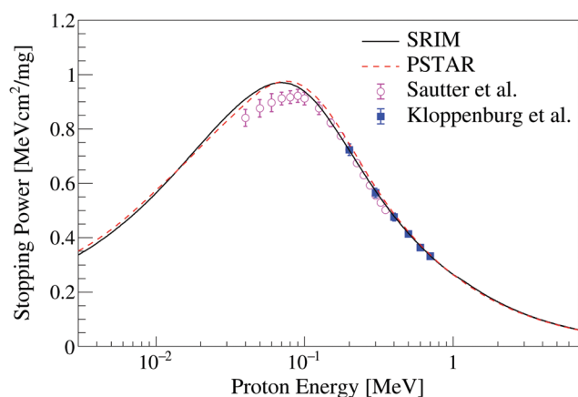
Fig. 6 Proton stopping power in PVT as calculated by SRIM (black curve) and PSTAR (red dashed curve) libraries. Only two measurements exist in the literature from Kloppenborg et al. (filled blue squares) and Sautter et al. (open pink circles).
