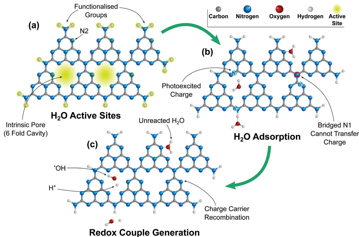
Fig. 8 Schematic diagram of g\text{-C}_3\text{N}_4 (tri- s -triazine (heptazine)) showing (a) \text{H}_2\text{O} adsorption sites, highlighted in yellow (b) \text{H}_2\text{O} adsorption onto g\text{-C}_3\text{N}_4 active sites, and electron trapping due to the bridged N1 preventing electron transfer between structural elements. 145 (c) Subsequent dissociation of \text{H}_2\text{O} into \cdot\text{OH}/\text{O}^+ redox couple where sufficient charge carriers are available.
