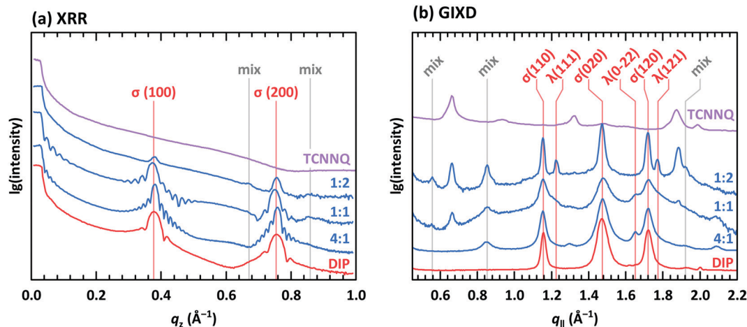
Fig. 8 (a) X-ray reflectivity (XRR) and (b) grazing incidence X-ray diffraction (GIXD) measurements for single component and co-deposited films of DIP and TCNNQ. The peaks donated as \sigma(\lambda) are related to phases containing upright standing (lying) DIP molecules. Peaks marked as “mix” are attributed to the formed mixed crystal. Corresponding respective reciprocal space maps are shown in ESI† (see Fig. S1).
