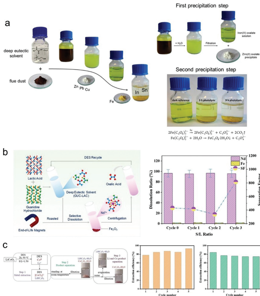
Fig. 9 (a) Schematic diagram of leaching and selective extraction of zinc, iron, indium, and tin using ChCl:oxalic acid DES-based two-step precipitation procedure (left); dilution of oxalate leachate and precipitation of white zinc oxalate next to the green-colored filtrate in the first precipitation step (upper right); photograph and reaction formulations of photolysis of iron(III) oxalate solution using a UV lamp in the second precipitation step (lower right). Reprint with permission from ref. 161. Copyright © 2019, American Chemical Society. (b) Schematic diagram of selectively leaching neodymium from end-of-life NdFeB permanent magnets by guanidine hydrochloride:lactic acid DES (left) and the recycling performance of the DES (right). Reprint with permission from ref. 130. Copyright © 2020, American Chemical Society. (c) Schematic diagram of the one-pot extraction process using ChCl:oxalic acid DES for the recovery of lithium and cobalt from LiCoO 2 and the recycling performance of DES for Li extraction (middle) and Co extraction (right). Reprint with permission from ref. 163. Copyright © 2021, American Chemical Society.
