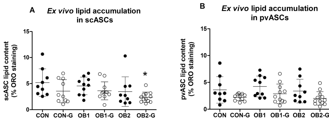
Fig. 4 Quantification of intracellular lipid accumulation in ex vivo adipocyte-differentiated subcutaneous (panel A) and perirenal visceral (panel B) ASCs (scASCs and pvASCs, respectively) is shown. Intracellular lipid droplets were stained with Oil Red O and staining was quantified with image analysis. Only adipogenic media (AM)-treated cultures were included in this analysis, as control media (CM) cultures typically contained no intracellular lipid droplets that became visible upon staining (also refer to ESI Fig. S2†). For both panels, each data point represents data for one animal ( n = 9 – 12 per dietary group). Black circles denote animals that did not receive GRT, while open circles denote animals that received GRT. Data was analysed using one-way ANOVA and Tukey's multiple comparisons post-hoc test. * p < 0.05 relative to CON.
