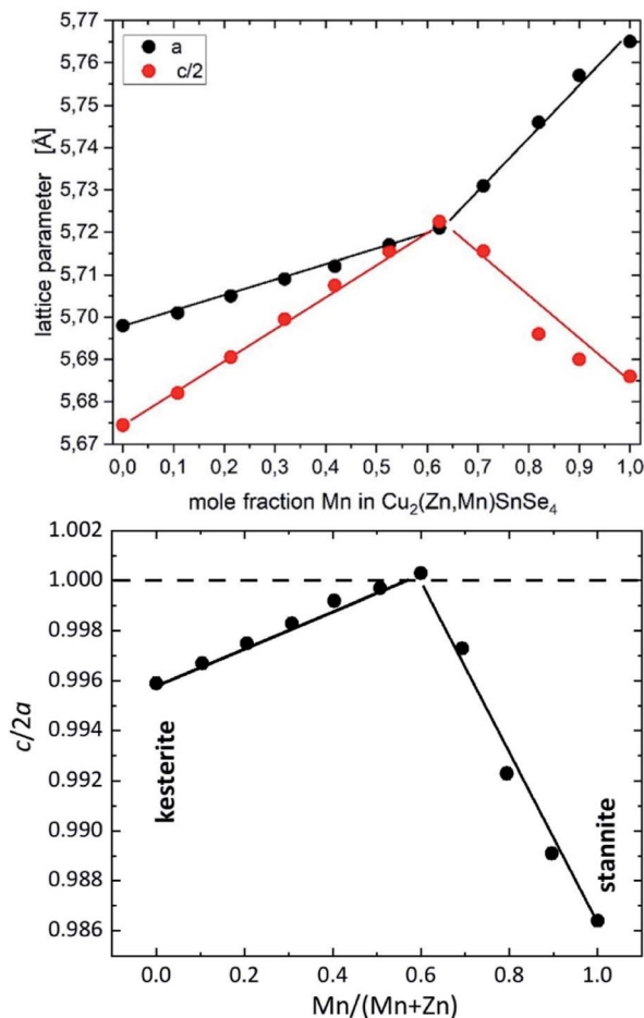
Fig. 3 Lattice parameters a and c (top) and tetragonal distortion c / 2a (bottom) of \text{Cu}_2(\text{-Zn}_x\text{Mn}_{1-x})\text{SnSe}_4 mixed crystals depending on the chemical composition. The lines are guides for the eye.
