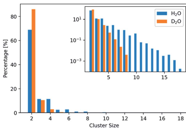
Fig. 2 Distribution of the number of ions per found cluster in light and heavy water. The distributions are normalized based on the total number of clusters found in the respective solvent. Two times more clusters (consisting of N(\text{ions}) > 2 ) were found in H 2 O compared to D 2 O.
