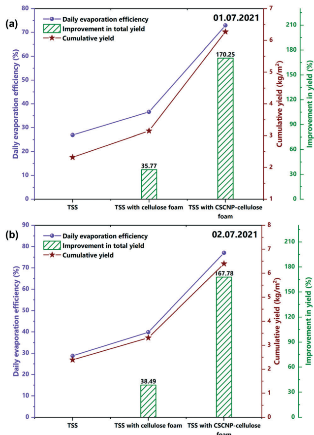
Fig. 12 (a and b) Average evaporation efficiency and enhancement in full day water yield of the unmodified, CF-modified and CSCNP-CF modified TSS on 1st and 2nd July, 2021.
