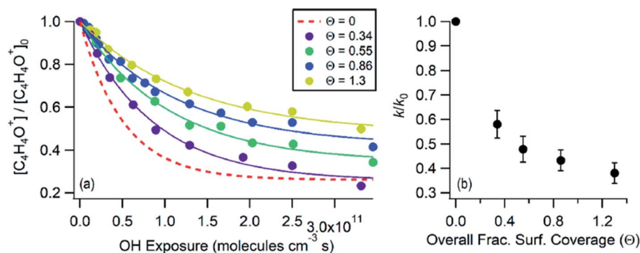
Fig. 14 (a) Decay in normalized tricarballic acid signal, measured as the C_4H_4O^+ fragment by aerosol mass spectrometry, as a function of OH exposure for varying overall fractional surface coverage ( \theta ) by SDS. \theta is calculated as a weighted average across all particle size bins in the polydisperse aerosol population. The solid lines are fits to the equation I/I_0 = I_0 + (1 - I_0)e^{-k[OH]t} , where I is the C_4H_4O^+ signal, I_0 is the C_4H_4O^+ signal at zero OH exposure, k is the effective second-order rate constant, and [OH]t is the OH exposure. The dashed red line is the fit line for tricarballic acid particles without SDS (data points not shown). (b) Rate constants for tricarballic acid decay in SDS-coated aerosol particles, normalized by the rate constant k_0 for particles without SDS. Reprinted with permission from J. A. Faust and J. P. D. Abbatt, Organic Surfactants Protect Dissolved Aerosol Components against Heterogeneous Oxidation, J. Phys. Chem. A , 2019, 123 , 2114–2124. Copyright 2019 American Chemical Society.
