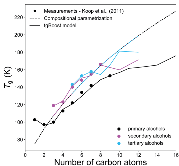
Fig. 4 T_g values of primary alcohols (black), secondary alcohols (magenta), and tertiary alcohols (light blue) as a function of the number of carbons of the n -alkyl chain. The markers represent the available experimental measurements, 7 the solid lines represent the predicted values by the tgBoost model, and the dashed lines represent the T_g predictions by the compositional parameterization. 8 Note that primary alcohols have a terminal –OH group, and secondary and tertiary alcohols have one –OH group placed on the second and third carbon atoms of the alkyl chain, respectively.
