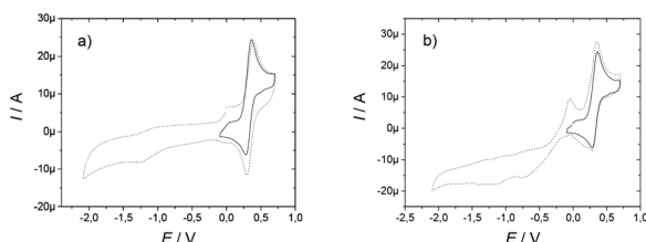
Fig. 2 CV curves of 0.5 mM CH 3 CN solutions (+0.1 TBAP) of (a) [L 1 -Eu] 3+ and (b) [L 2 -Eu] 3+ at a carbon electrode. T = 298 K, scan rate = 0.1 V s −1 . All values reported with respect to the regular Fc + /Fc redox couple that was used as an external reference.
