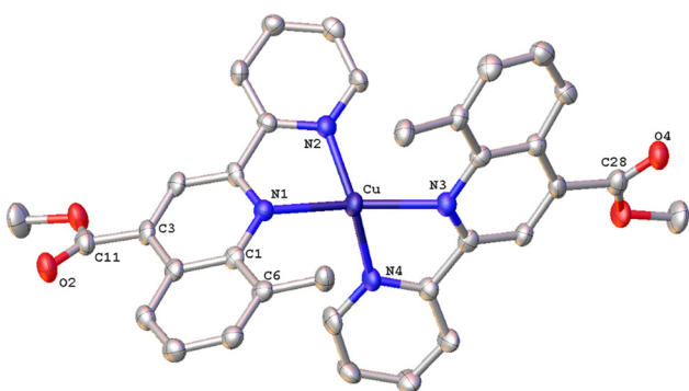
Fig. 7 Molecular structure of the cation of complex [\text{Cu}(8\text{-Mepqame})_2][\text{PF}_6] \cdot (2\{7\text{-C}_5\text{H}_{12}\}) \cdot \text{CHCl}_3 ; ellipsoids are plotted at the 50% probability level. H atoms, except those in the COOH groups, and the co-crystallized solvents are omitted for clarity.
