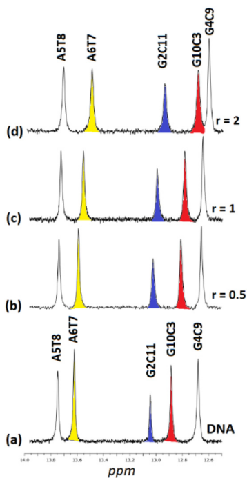
Fig. 9 Part of the ^1\text{H} NMR spectra of the \text{d}(5' \text{-CGCGAATTCGCG-}3')_2 (a) free, and upon addition of (6) \text{Cl}_4 at r = 0.5, 1 and 2 , (b–d), showing the imino protons of the W.–C. hydrogen bonds.
