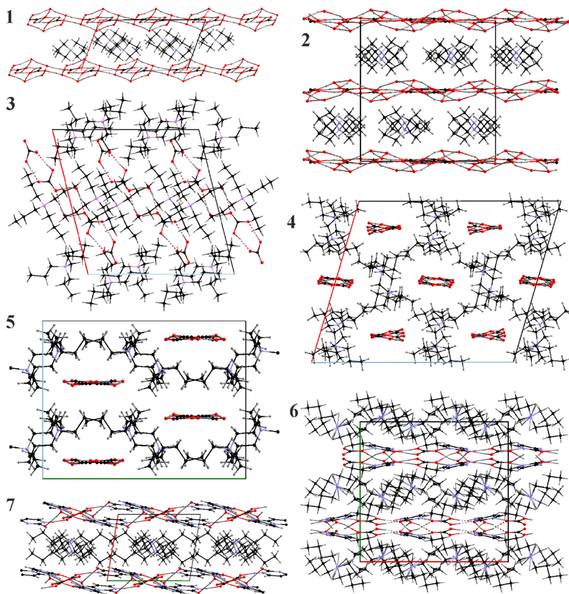
Fig. 3 Packing of the cations and the anionic fragments in the crystal structures of [\text{N}_{2222}][\text{HCO}_3] \cdot 3\text{H}_2\text{O} ( 1 ), [\text{N}_{2222}][\text{H}(\text{HCO}_3)_3] \cdot 5\text{H}_2\text{O} ( 2 ), [\text{N}_{3333}][\text{HCO}_3] \cdot 0.5\text{H}_2\text{O} ( 3 ), [\text{N}_{3333}][\text{H}(\text{HCO}_3)_2] ( 4 ), [\text{N}_{3333}][\text{tpa}](\text{H}_2\text{CO}_3)_2 ( 5 ), [\text{N}_{4444}][\text{H}(\text{Cyt})(\text{HCO}_3)] \cdot \text{H}_2\text{O} ( 6 ) and [\text{N}_{4444}][\text{H}_2(\text{Cyt})_2(\text{HCO}_3)] \cdot \text{H}_2\text{O} ( 7 ).
