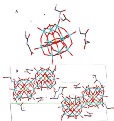
Fig. 3 The molecular (A) and crystal (B) structure of compound (\text{HGlGly})_3[\text{PMo}_{12}\text{O}_{40}] \cdot 3\text{H}_2\text{O} (3).
